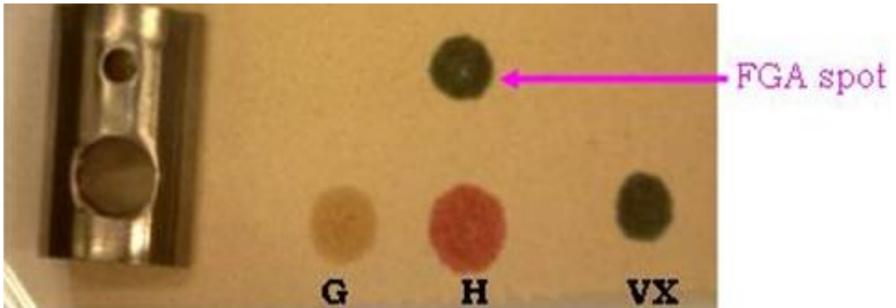
Liquid FGA on M8 Paper – 10 Seconds
