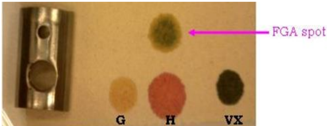
Liquid FGA on M8 Paper – 10 Minutes
